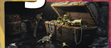
Stormbringer
